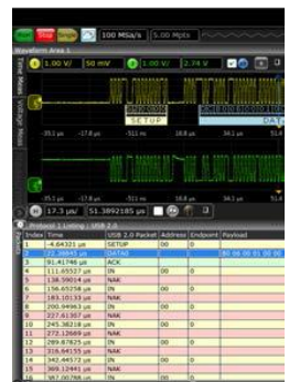
Protocol Decode
